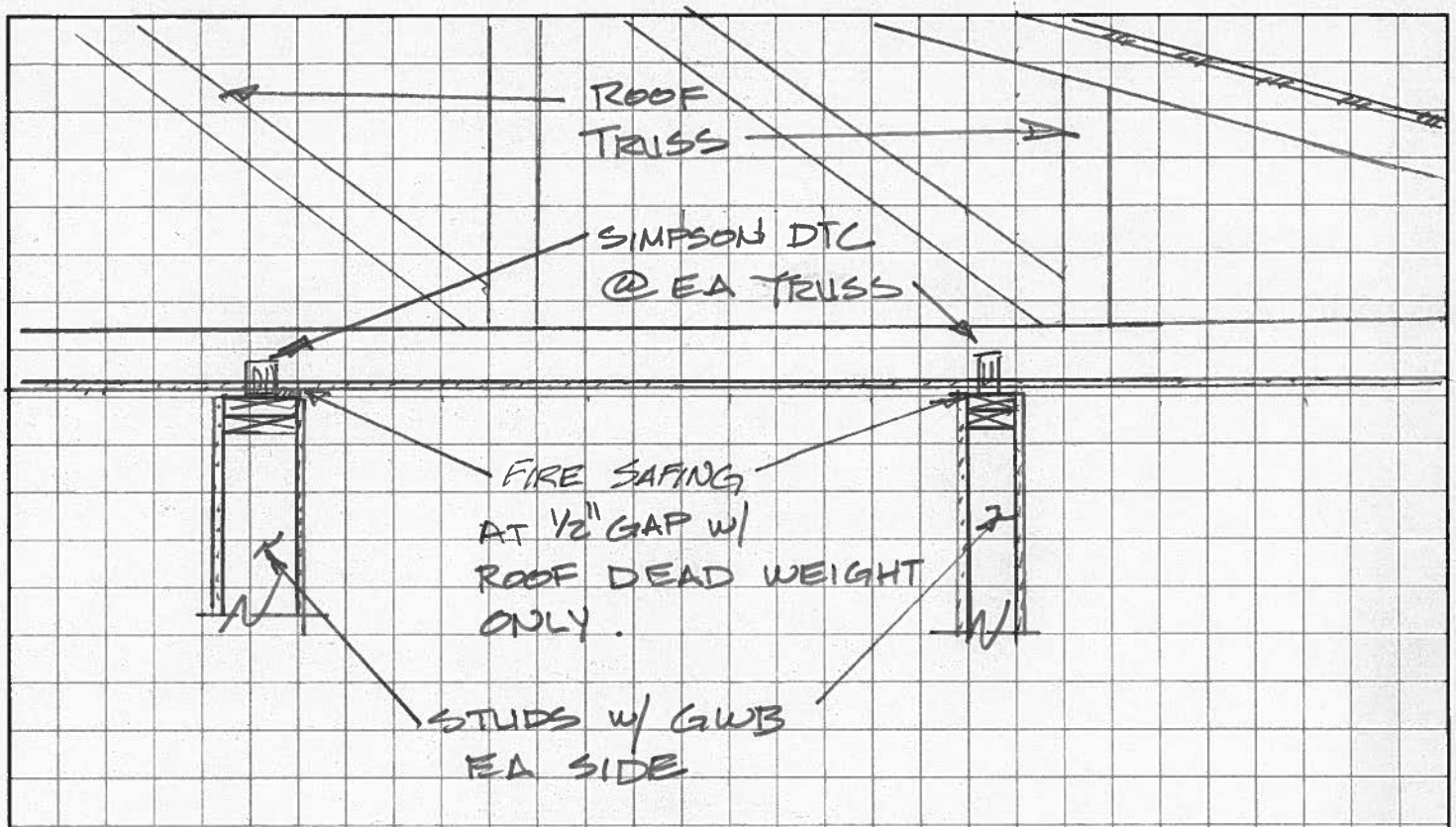
① ROOF TRUSS @ LIFT WALLS ON S40Z
