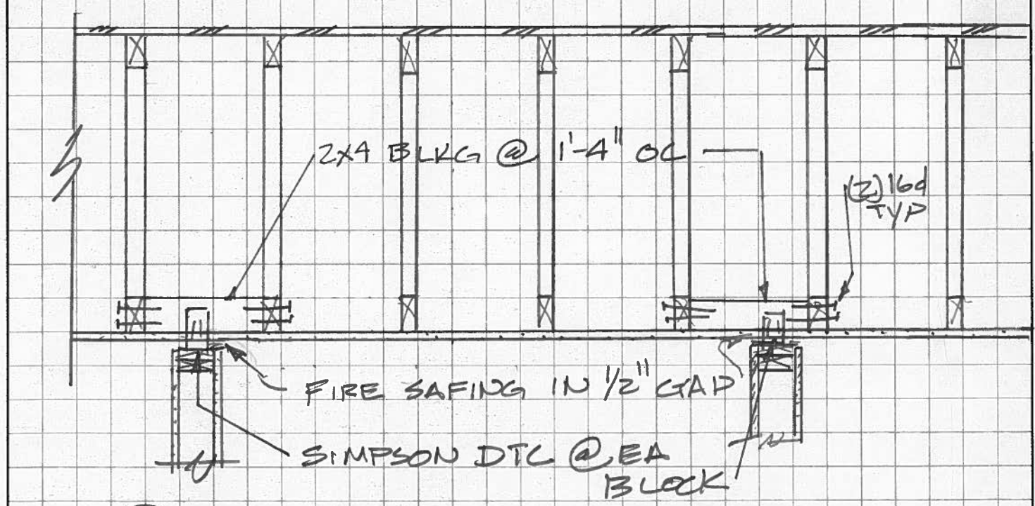
② ROOF TRUSSES @ LIFT WALLS
